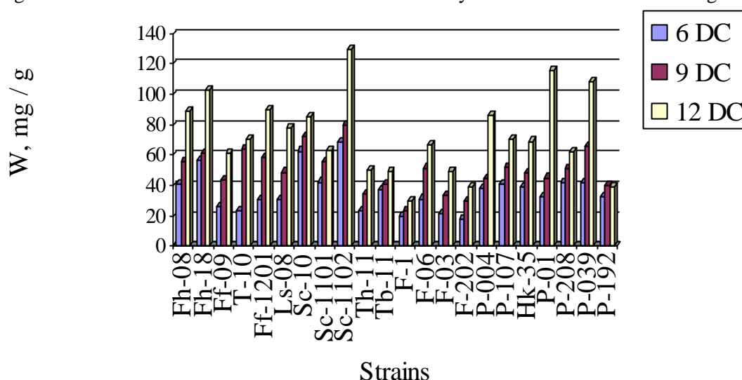
Fig. 2. The total content of polyphenols of mycelium of strains of Basidiomycetes on 6 th , 9 th and 12 th days of cultivation
