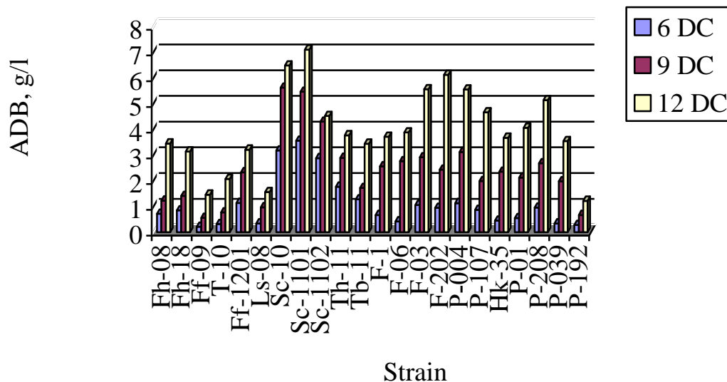
Fig. 1. Accumulation of absolute dry biomass of strains of Basidiomycetes on the 6 th , 9 th and 12 th days of cultivation
